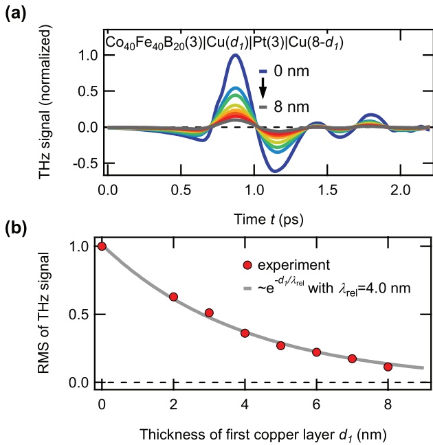
Figure 4. Role of the interface in THz-emission studies. (a) THz waveforms emitted from \text{Co}_{40}\text{Fe}_{40}\text{B}_{20}|Cu(d_1)|Pt(3)|Cu(8-d_1) structures with fixed \text{Co}_{40}\text{Fe}_{40}\text{B}_{20} and Pt thicknesses of 3 nm and d_1 ranging from 0 to 8 nm. (b) THz-signal amplitudes (RMS) versus d_1 together with a single exponential fit \propto \exp(-d_1/\lambda_{\text{rel}}) with \lambda_{\text{rel}} = (4.0 \pm 0.1) nm. The experimental data is normalized by the maximum signal amplitude.
