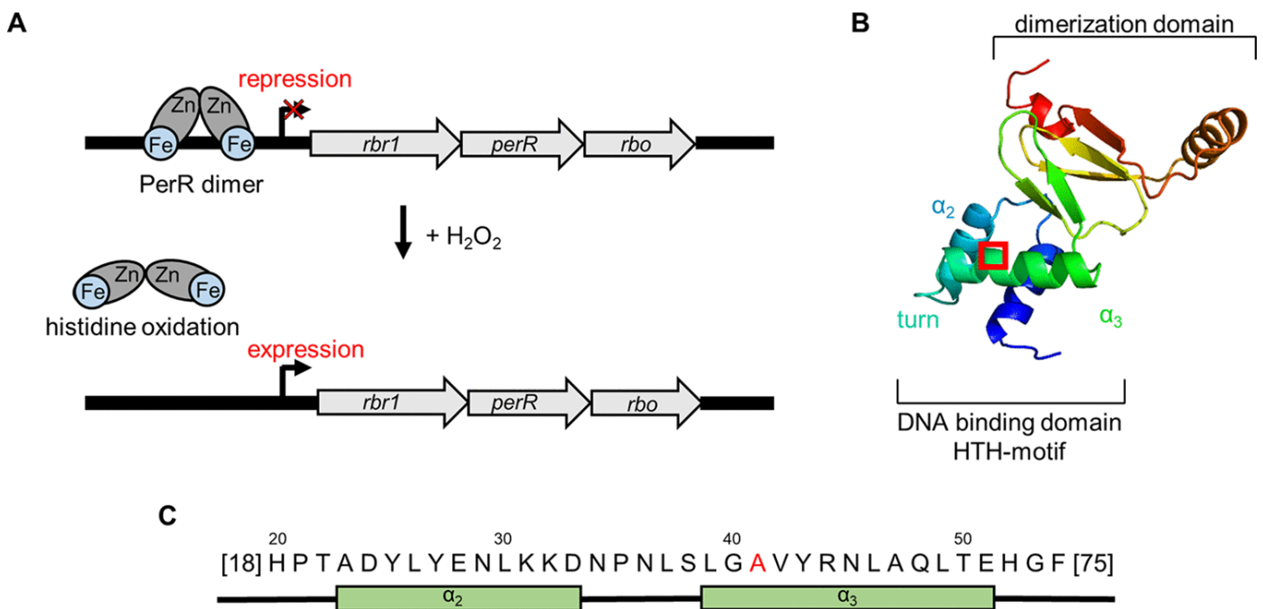
FIG 1 DNA binding of PerR. (A) Mode of PerR function shown schematically. PerR bound to the DNA represses the expression of the rbr1 operon. H_2O_2 treatment leads to PerR oxidation, a conformational change, and the release of the DNA promoter, resulting in the expression of the rbr1 operon. (B) Structure of C. difficile 630 \Delta erm PerR deduced from the homologue of B. subtilis . The DNA binding site, including the helix-turn-helix (HTH) motif and the dimerization domain, is marked. The location of the amino acid exchange is marked by a red box. (C) Amino acid sequence of the DNA binding site of C. difficile 630 \Delta erm PerR. The T41A mutation is marked in red.
