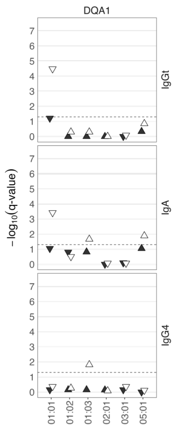
Supplementary Fig. 3: HLA-DQA alleles are associated with low or high anti-TSST-1 IgGt and IgA antibody levels. HLA-DQA alleles were deduced from Illumina WGS data using the HLA-HD algorithm (n=402, dark gray) or predicted from genotyping array data using the Four-digit Multi-ethnic HLA v2 imputation panel (n=965, white). -\log_{10}(\text{q-value}) , negative decadic logarithm of the Benjamini-Hochberg (BH) adjusted p-value.
